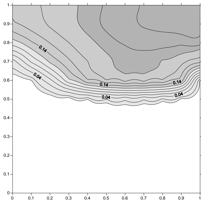
Figure 2b Redistribution of TCE after 7 days (Multiple layer of soil)
