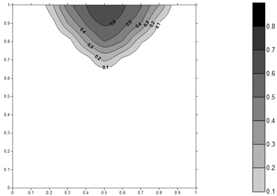
Figure 1a Injection of TCE for 3 hours (One type of soil)
