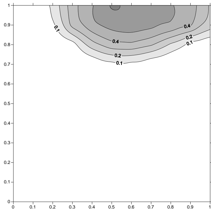
Figure 1b Injection of TCE for 3 hours (Multiple layer of soil)
